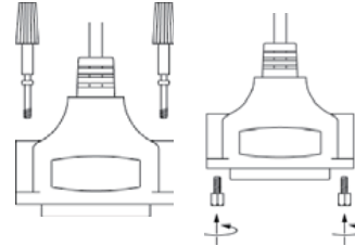
Bi-Directional Reversible Connector
