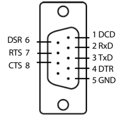
DB9 Male (CBL-M62M9x8-100 (OPT8D))
