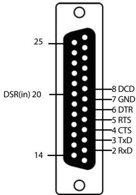
DB25 Female (OPT8A/S)
