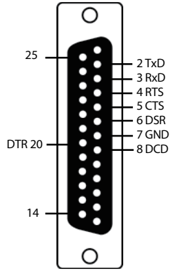
DB25 Male (OPT8B/CBL-M62M25x8-100 (OPT8C))
